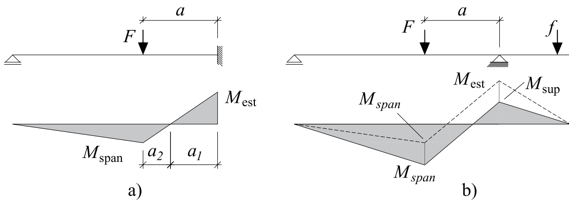
Figure 4 –Bending moments in structures with a) fully clamped support and b) partially clamped support.
