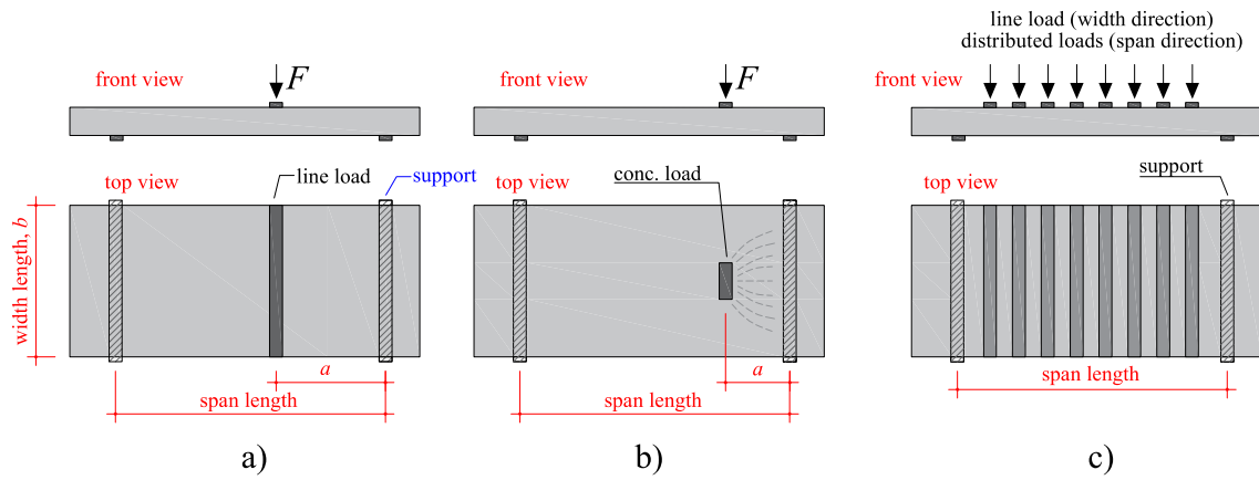
Figure 1 – Main types of loads on wide members: a) concentrated in the span length and distributed along the width; b) concentrated in the span and width directions (not included in the scope of this study) and c) distributed load in both span and width direction.
