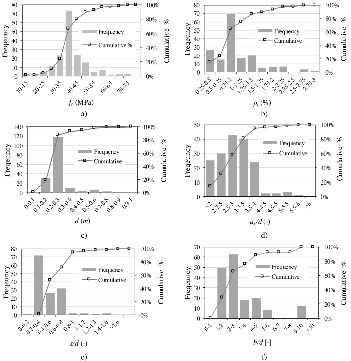
Figure 8 - Distribution of parameters in database: (a) concrete compressive strength f_c ; (b) longitudinal reinforcement ratio \rho_l ; (c) effective depth of the longitudinal reinforcement d ; (d) clear shear span to effective depth ratio a_v/d ; e) rebar spacing to effective depth ratio s/d ; f) member width to effective depth ratio b/d .
